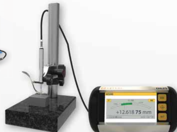
Probe P12D with output M8 connected on the D62S Standard
